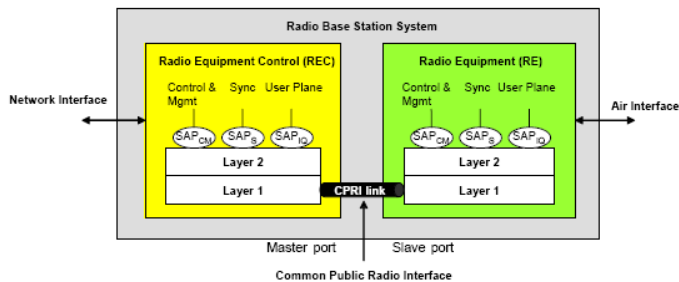
Figure 1. Illustration of the basic building blocks in a radio base station using CPRI.
